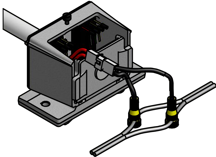
CONNECTION IN JUNCTION BOX WITH POSI TAP
