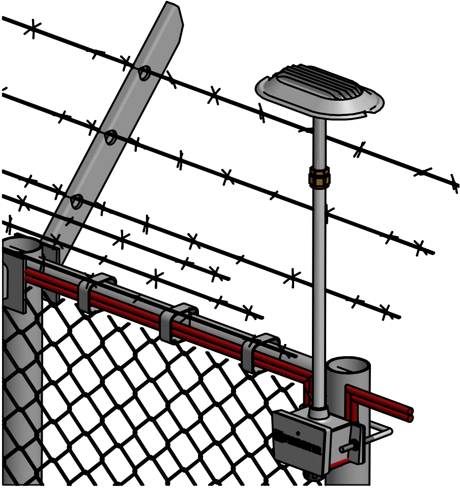
WIRE ATTACHED TO TOP RAIL
